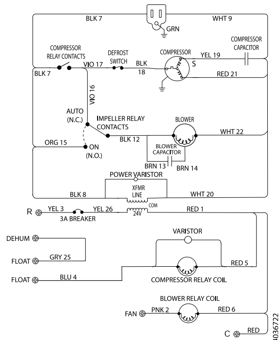
Santa Fe ULTRA120H Wiring Diagram
